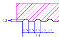
DETAIL-I GULF EXTRUSIONS (IDENTIFICATION MARK)
